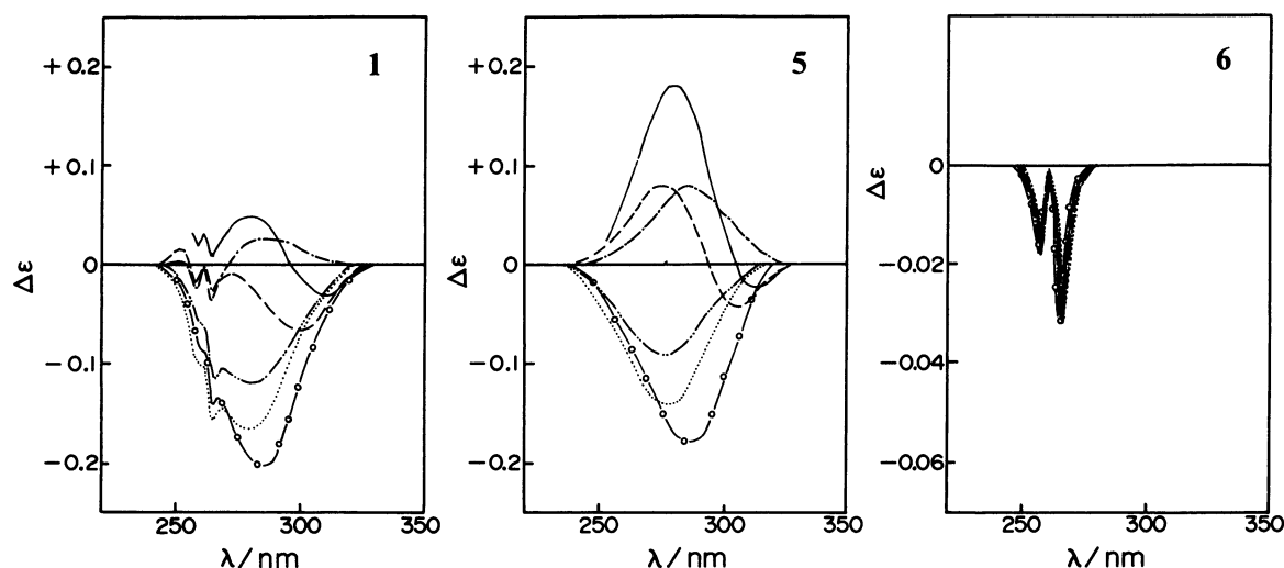
Fig. 6. CD curves of 1 , 5 , and 6 : — in carbon tetrachloride (a), --- in chloroform (b), -·-·- in diethyl ether (f), ..... in dioxane (g), ○-○ in acetonitrile (j), ..... in methanol (k).
