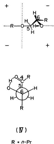
Fig. 8. The most stable conformation of 5 in the case that the intramolecular hydrogen bond is formed.
